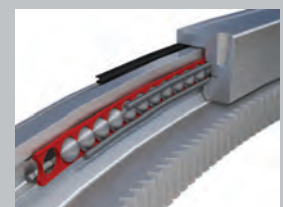
Wire Race
